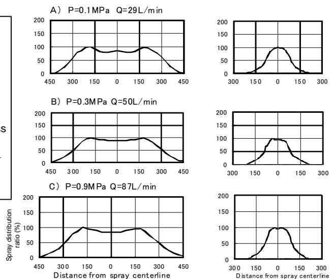
Spray distribution in width direction
