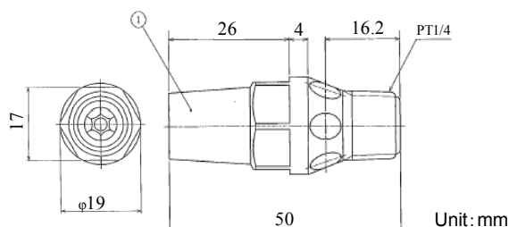
① Nozzle
