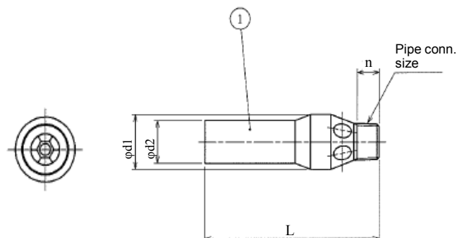
① Nozzle
