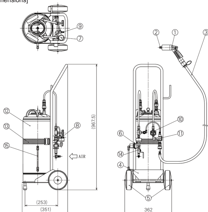
[Dimensions]
